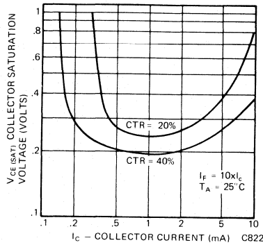
Fig. 14 Saturation Voltage vs. Collector Current
