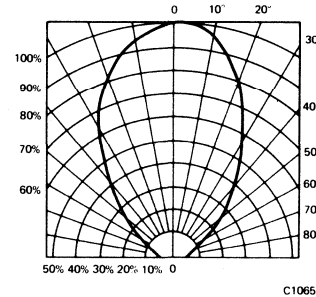
Fig. 3. Spatial Distribution (Note 2) for MV5753
