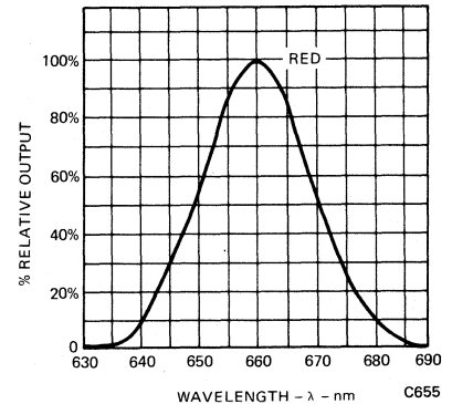
Fig. 5. Spectral Distribution
