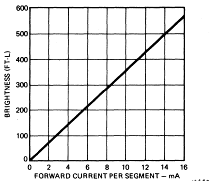
Figure 1 Brightness vs. Forward Current
