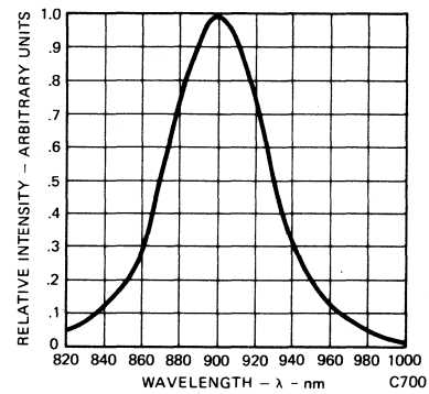
Fig. 6. Spectral Distribution
