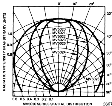
Fig. 4. Spatial Distribution
