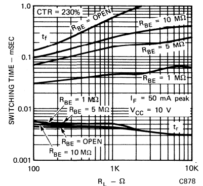
Fig. 9. Switching Times
