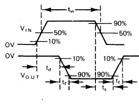
Fig. 11 Waveforms for Figure 7
