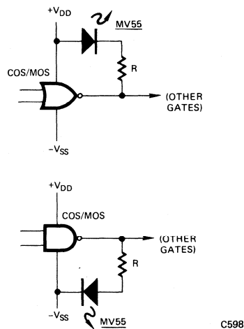
Fig. 5 MV55A Interfaced with COS/MOS
