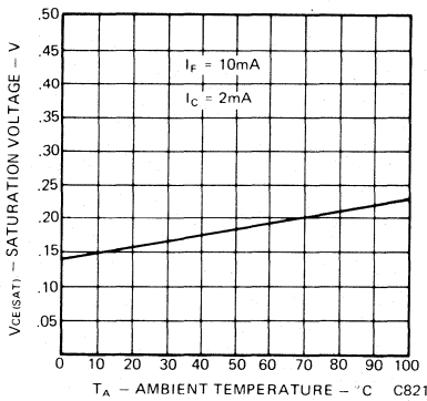
Fig. 13 Saturation Voltage vs. Temperature
