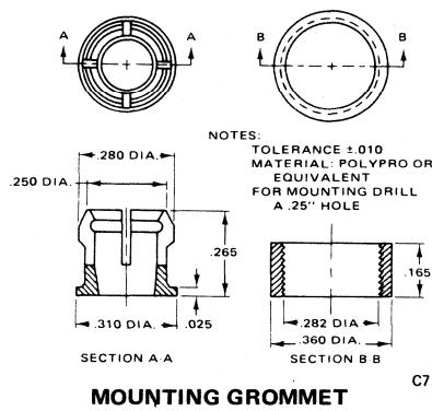
MOUNTING GROMMET
