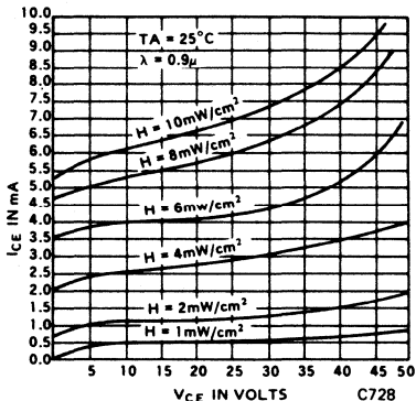
Fig. 1. Collector-Emitter Characteristics
