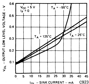
Fig. 4. Low Level Output Voltage vs. Sink Current
