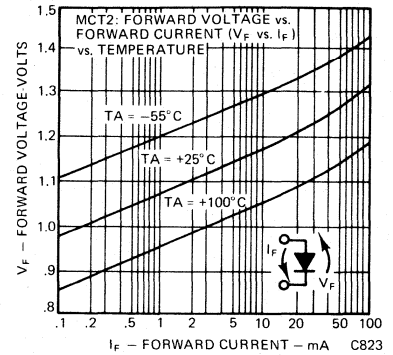
Fig. 15 Forward Voltage vs. Forward Current
