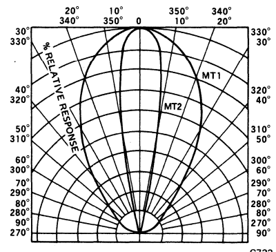
Figure 6 Angular Response
