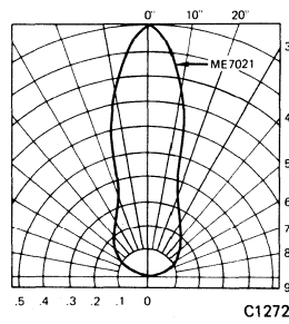
Fig. 5. Spatial Distribution (ME7021)
