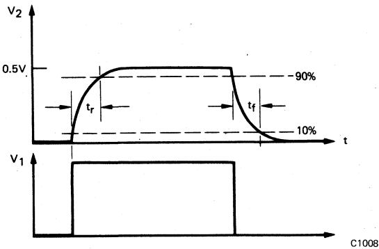
Figure 10 Non-Saturated Switching Waveforms
