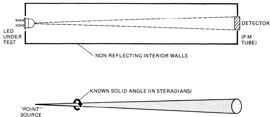
Fig. 3. Jigging for "I" Measurement
