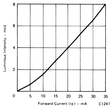
Fig. 3. Luminous Intensity vs. Forward Current (see Note 2)
