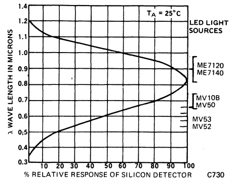
Figure 3 Spectral Response
