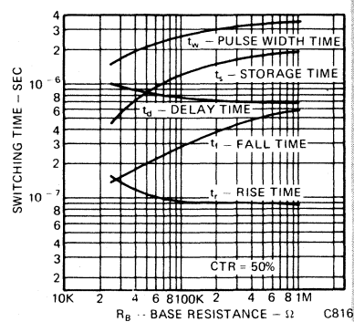
Fig. 3. Switching Time vs. Base Resistance
