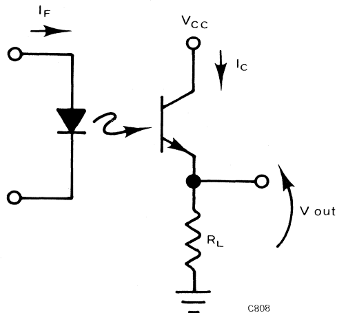
Circuit 1
