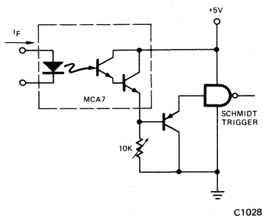
Circuit 1
