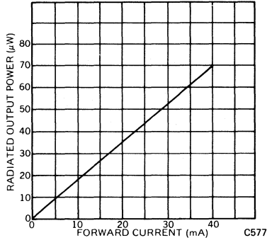
Figure 1 ROP vs. Forward Current
