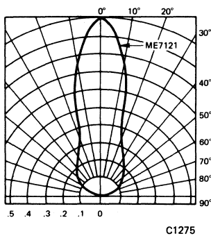
Fig. 4. Spatial Distribution (ME7121)
