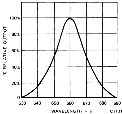
Fig. 5. Spectral Response
