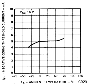
Fig. 10. MCL610—Negative-Going Threshold Current vs. Ambient Temperature
