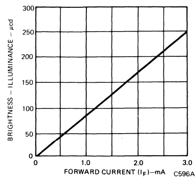
Fig. 3 Brightness vs. Forward Current
