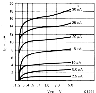
Fig. 4. Collector Current vs. Collector to Emitter Voltage
