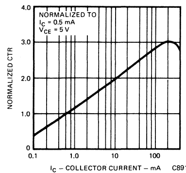
Figure 6. Normalized CTR vs. Collector Current
