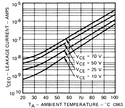
Figure 6 Leakage Current vs. Temperature vs. Collector Voltage
