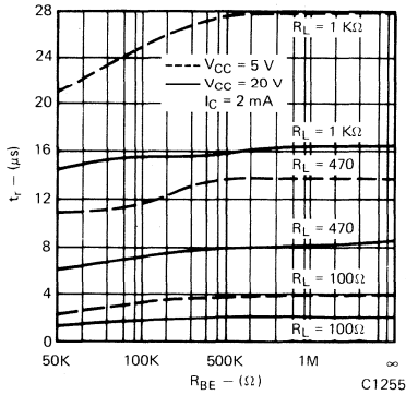
Fig. 15. Rise Time vs. Base to Emitter Resistance (non-saturated)
