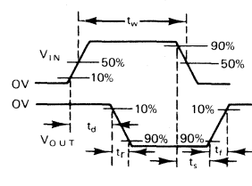
Fig. 6. Waveforms for Figure 3
