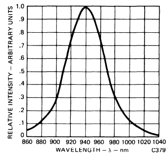
Fig. 6. Spectral Distribution
