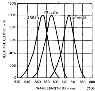
Fig. 2. Spectral Response
