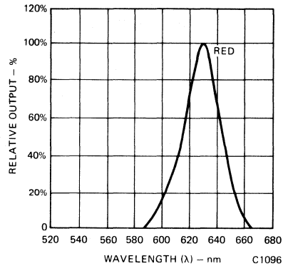
Fig. 2. Spectral Response
