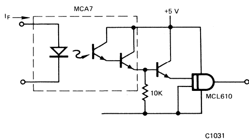
Circuit 4
