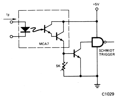
Circuit 2
