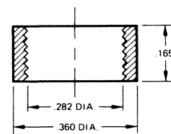
Fig. 5. Mounting Grommet MP51 (supplied on request only)
