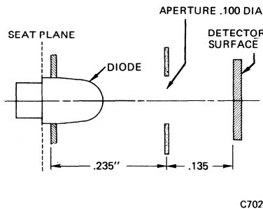
Fig. 8. Zone 1 Measurement
