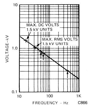
Fig. 9. Steady-State AC Voltage Limit of Isolation Dielectric
