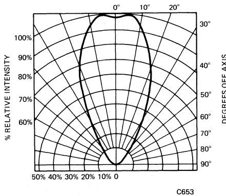
Fig. 3. Spatial Distribution
