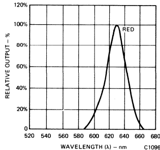
Fig. 2. Spectral Response
