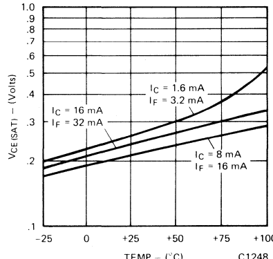
Fig. 9. Collector to Emitter Saturation Voltage vs. Temperature
