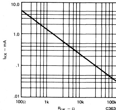
Fig. 5. Holding Current vs. Gate-Cathode Resistance
