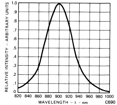
Fig. 6. Spectral Distribution
