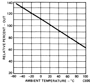
Fig. 5. % Relative Output vs. Temperature
