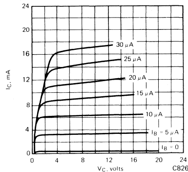
Fig. 10. Detector Typical h_f Curves
