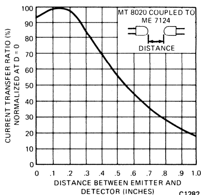
Fig. 5. Normalized Current Transfer Ratio vs. Distance Between Emitter and Detector MT8020 and ME7124.
