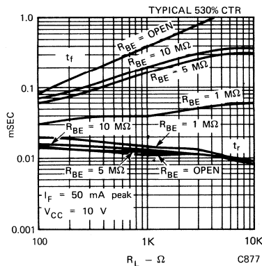
Fig. 8. Switching Times
