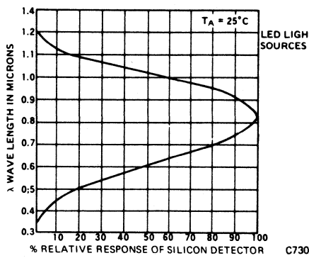
Fig. 2. Spectral Response
