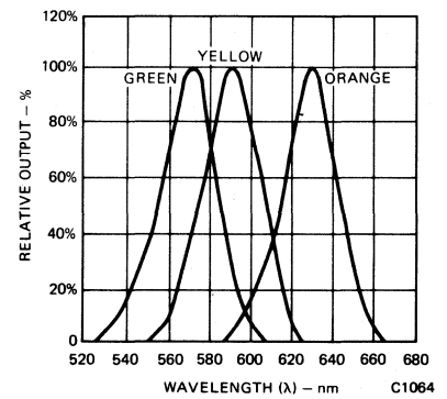
Fig. 3. Spectral Response
