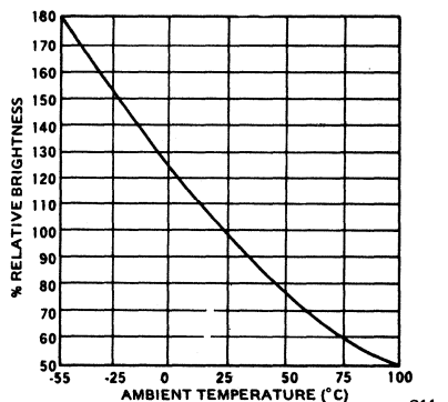
Figure 2 Brightness vs. Temperature
