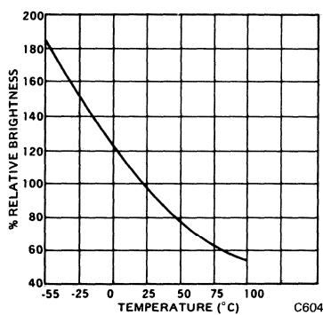
Fig. 1. Brightness vs. Temperature
