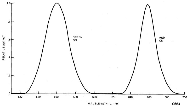
Fig. 5. Spectral Distribution
