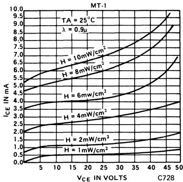
Figure 1 Collector-Emitter Characteristics
