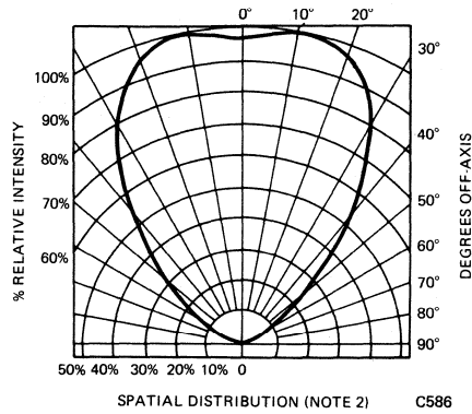
Fig. 3. Spatial Distribution (Note 2)
