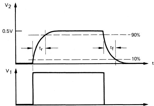
Figure 9. Non-Saturated Switching Waveforms
