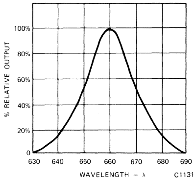
Fig. 3. Spectral Response
